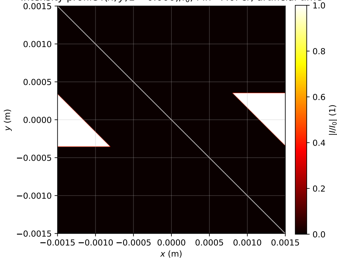
Intensity profile I(x, y, z = 0.000)/I_0 , P_{in}=7.0P_{cr} , artificial time
